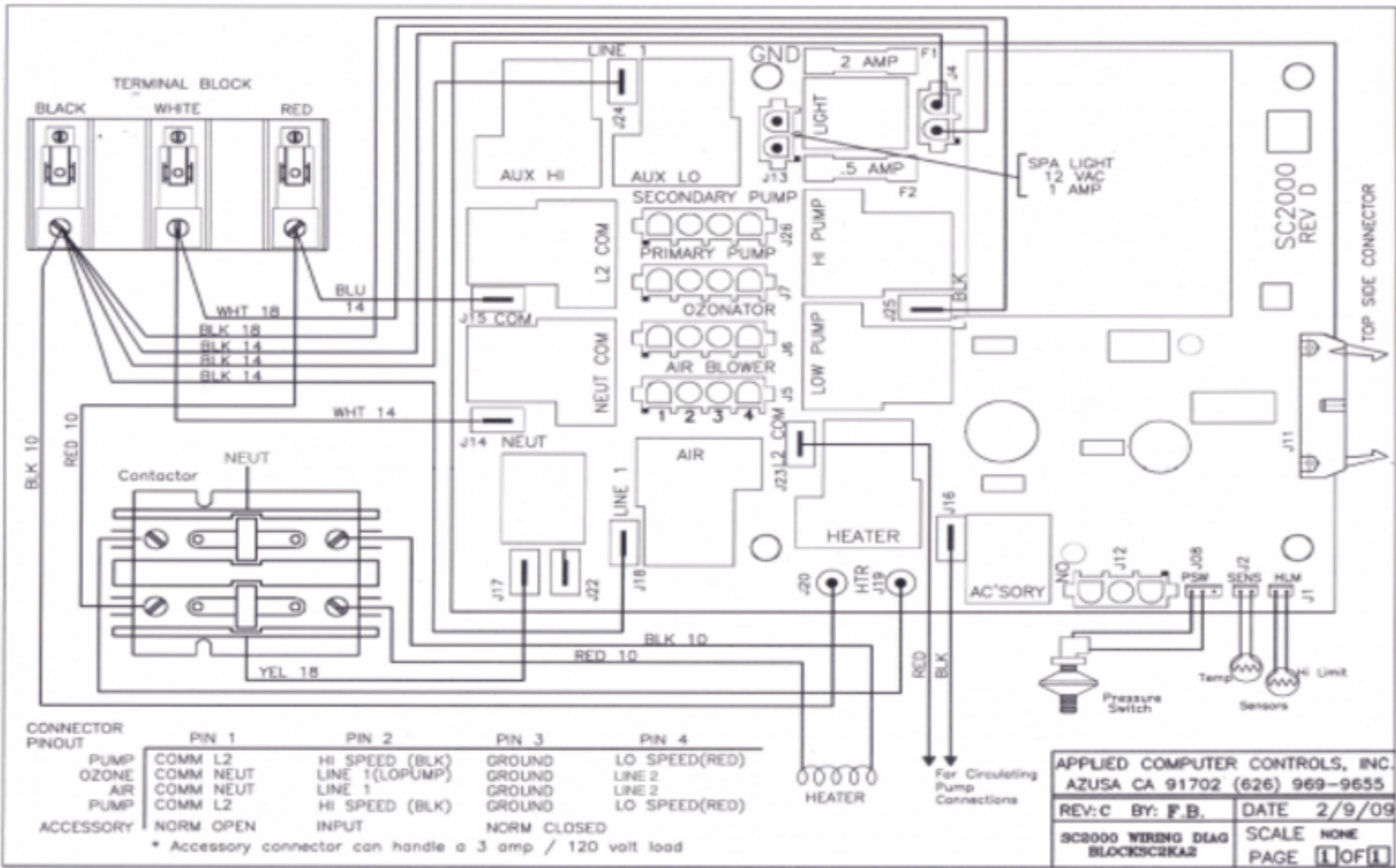
WIRING DIAGRAM FOR SMTD 2000 W/CIRCULATING PUMP
